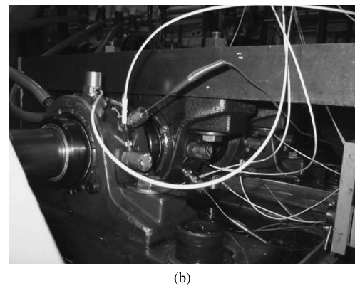
FIGURE 5. Illustration of the (a) bearing test rig and (b) vibration sensor placement of the IMS dataset [31].
