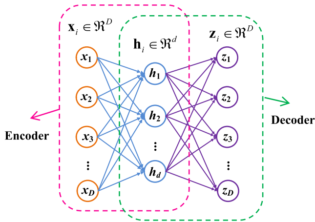
Fig. 1. The structure of an autoencoder.
