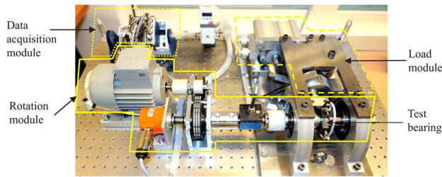
FIGURE 4. PRONOSTIA testbed (Department of Automatic Control and Micro-Mechatronic Systems (AS2M), Franche-Comté Electronique Mécanique [29].
