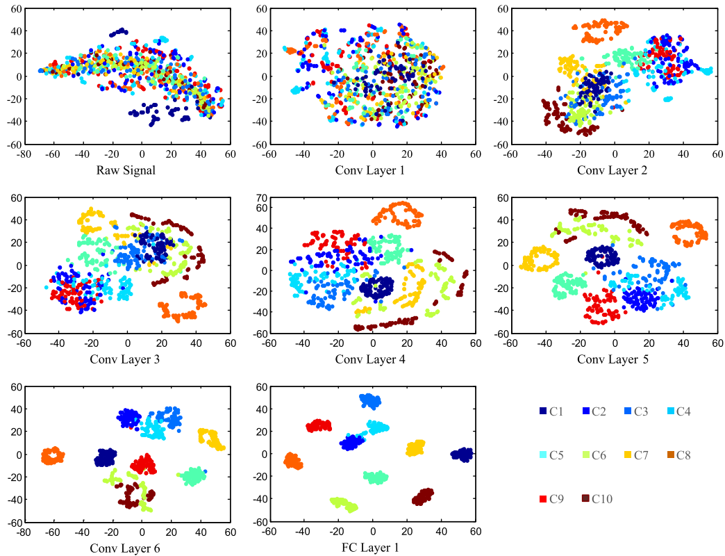
FIGURE 12. Feature visualization via t-SNE: feature representations for all test signals extracted from raw signal, six convolutional layers and the last fully connected layer respectively [111].
