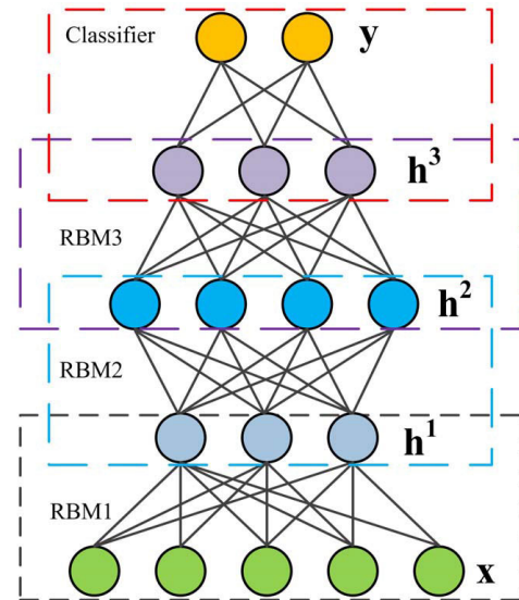
FIGURE 9. Architecture of DBN [135].
