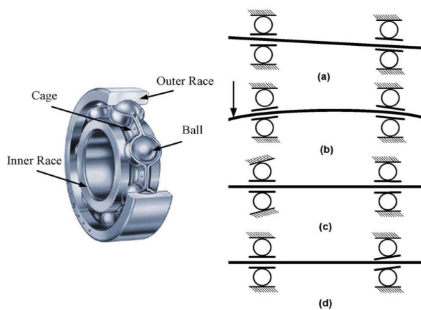
FIGURE 1. Structure of a rolling-element bearing with four types of common scenarios of misalignment that are likely to cause bearing failures: (a) misalignment (out-of-line), (b) shaft deflection, (c) crooked or tilted outer race and (d) crooked or tilted inner race [8].
