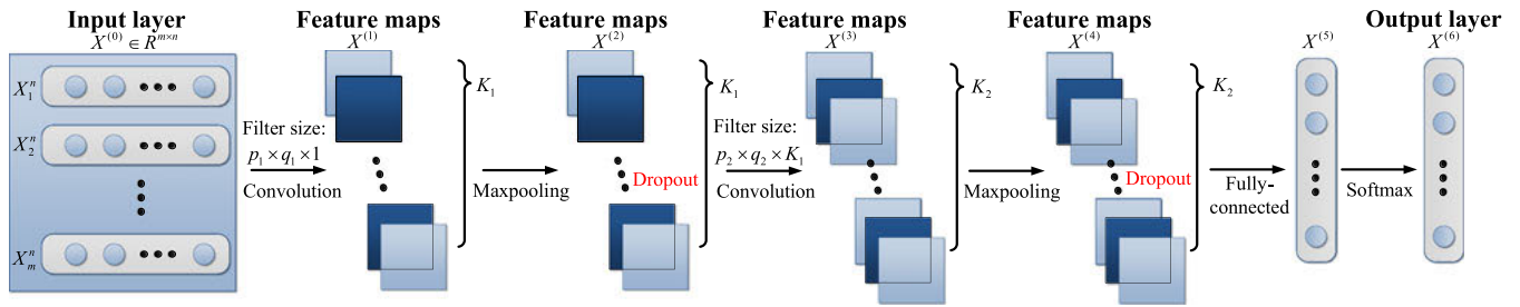
FIGURE 7. Architecture of the CNN-based fault diagnosis model [108].
