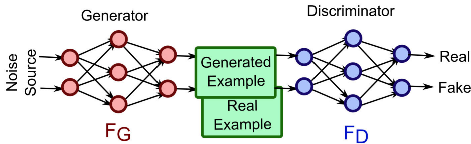
FIGURE 11. Architecture of GAN [148].
