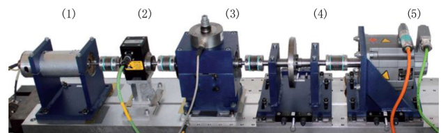
FIGURE 3. Modular test rig collecting the Paderborn bearing dataset consisting of (1) an electric motor, (2) a torque-measurement shaft, (3) a rolling bearing test module, (4) a flywheel, and (5) a load motor [27].
