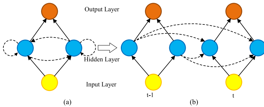
FIGURE 10. Architecture of (a) RNN, and (b) RNN over a time step [143].
