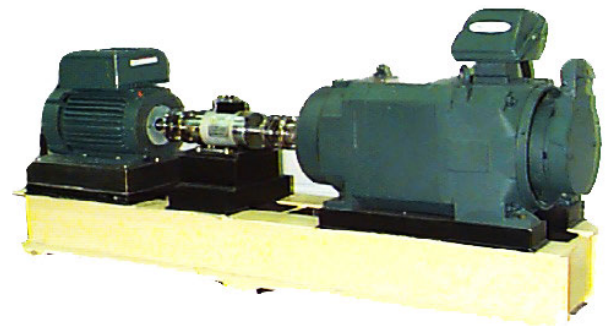
FIGURE 2. Experimental setup for collecting the CWRU bearing dataset [26].
